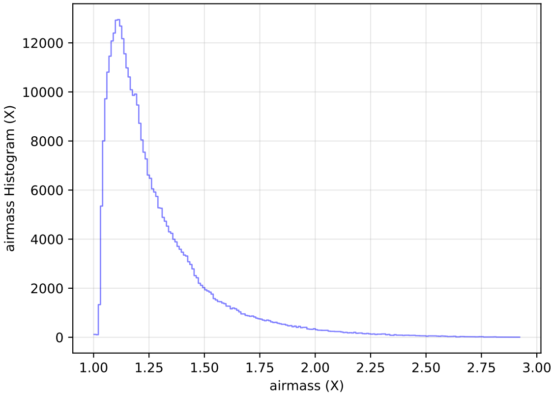
extra_ss_neo7_v3.4_10yrs WFD y band: airmass Histogram
