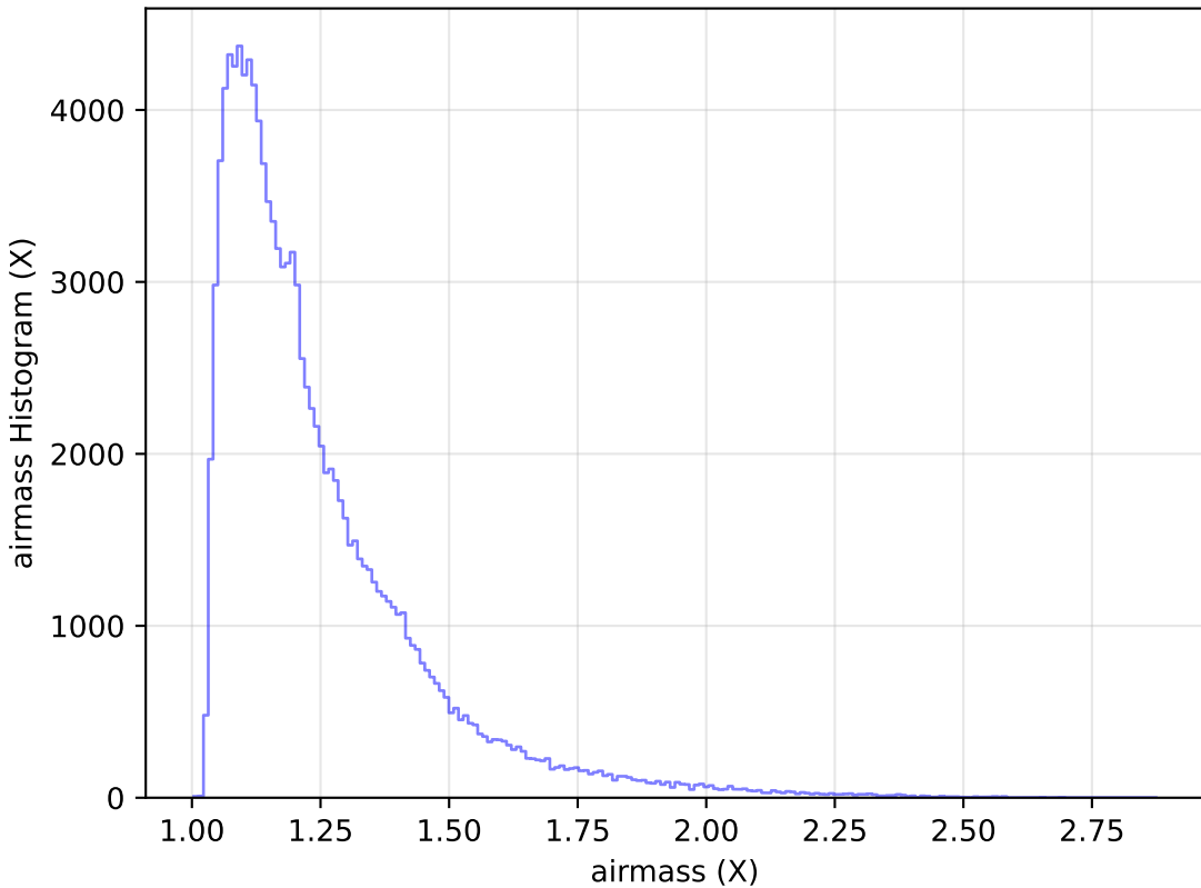
extra_ss_neo7_v3.4_10yrs WFD u band: airmass Histogram
