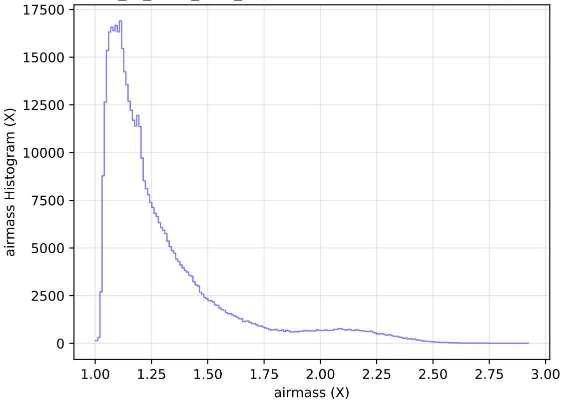
extra_ss_neo7_v3.4_10yrs WFD r band: airmass Histogram
