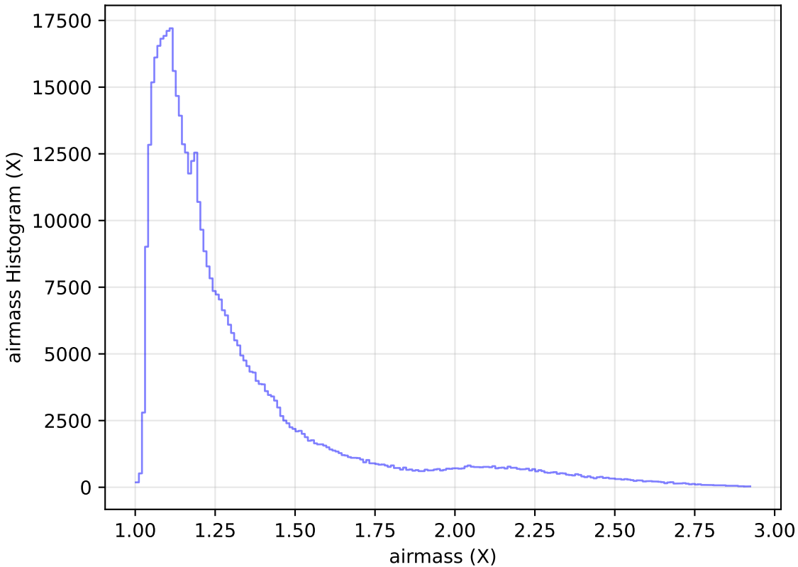
extra_ss_neo7_v3.4_10yrs WFD i band: airmass Histogram
