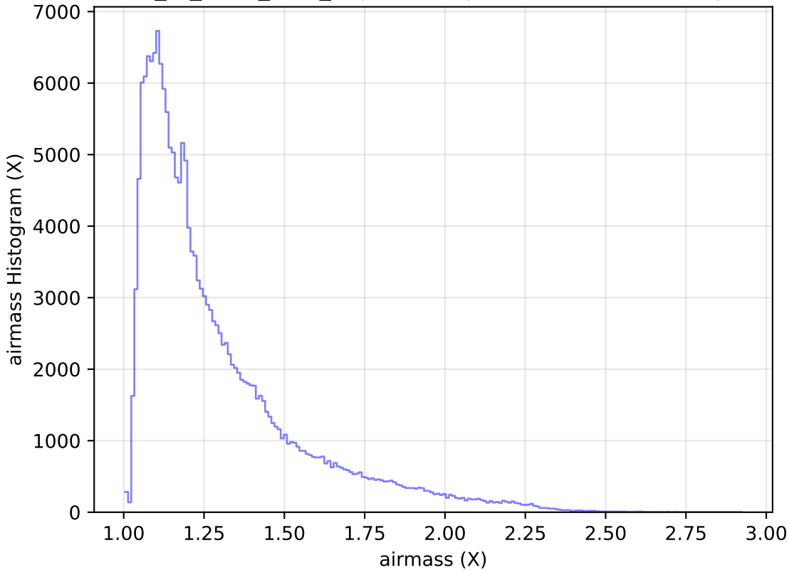
extra_ss_neo7_v3.4_10yrs WFD g band: airmass Histogram
