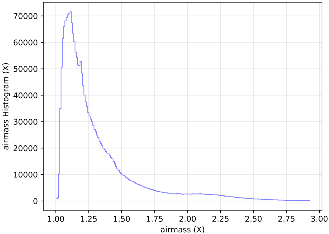
extra_ss_neo7_v3.4_10yrs WFD all bands: airmass Histogram
