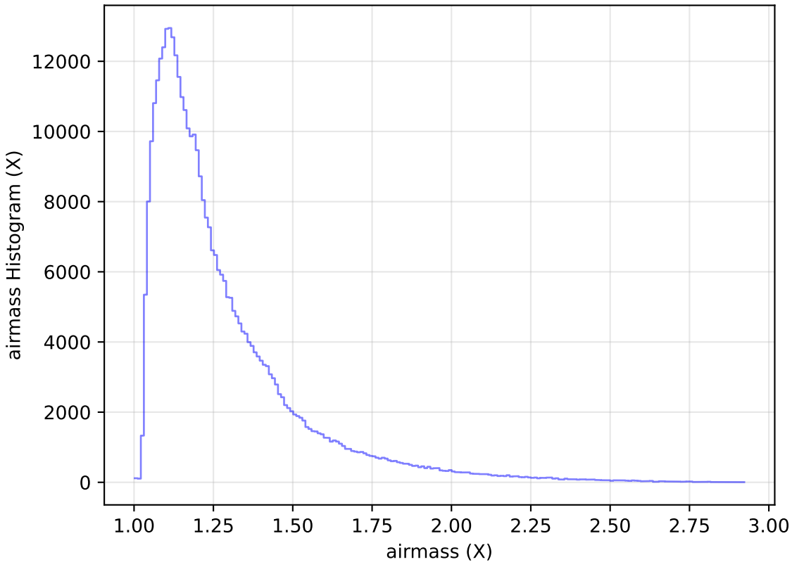
extra_ss_neo7_v3.4_10yrs All sky y band: airmass Histogram
