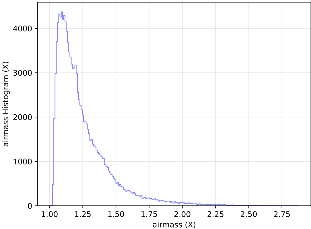
extra_ss_neo7_v3.4_10yrs All sky u band: airmass Histogram
