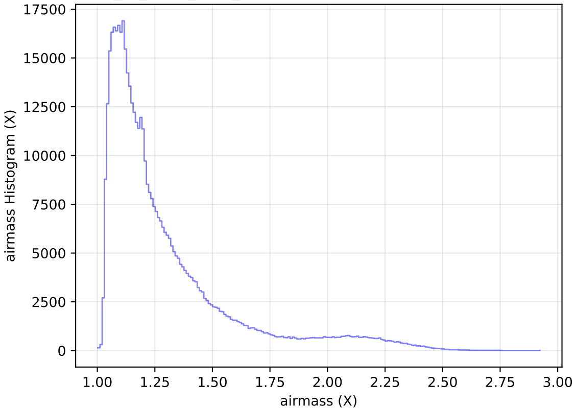
extra_ss_neo7_v3.4_10yrs All sky r band: airmass Histogram
