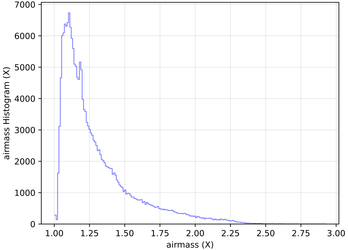
extra_ss_neo7_v3.4_10yrs All sky g band: airmass Histogram
