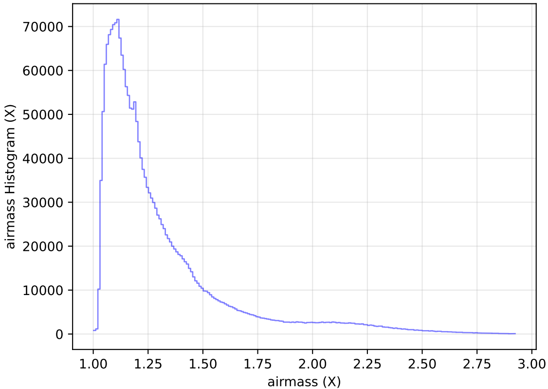
extra_ss_neo7_v3.4_10yrs All sky all bands: airmass Histogram
