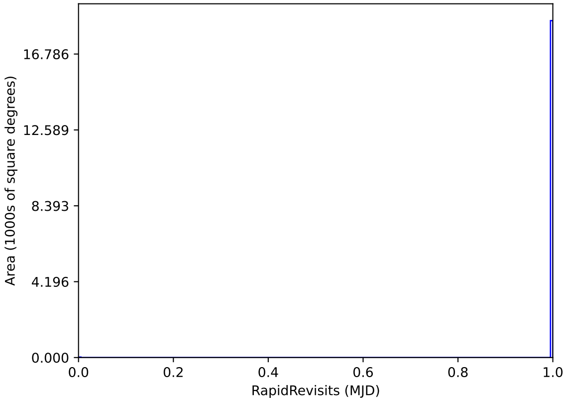
extra_ss_neo7_v3.4_10yrs WFD: RapidRevisits
