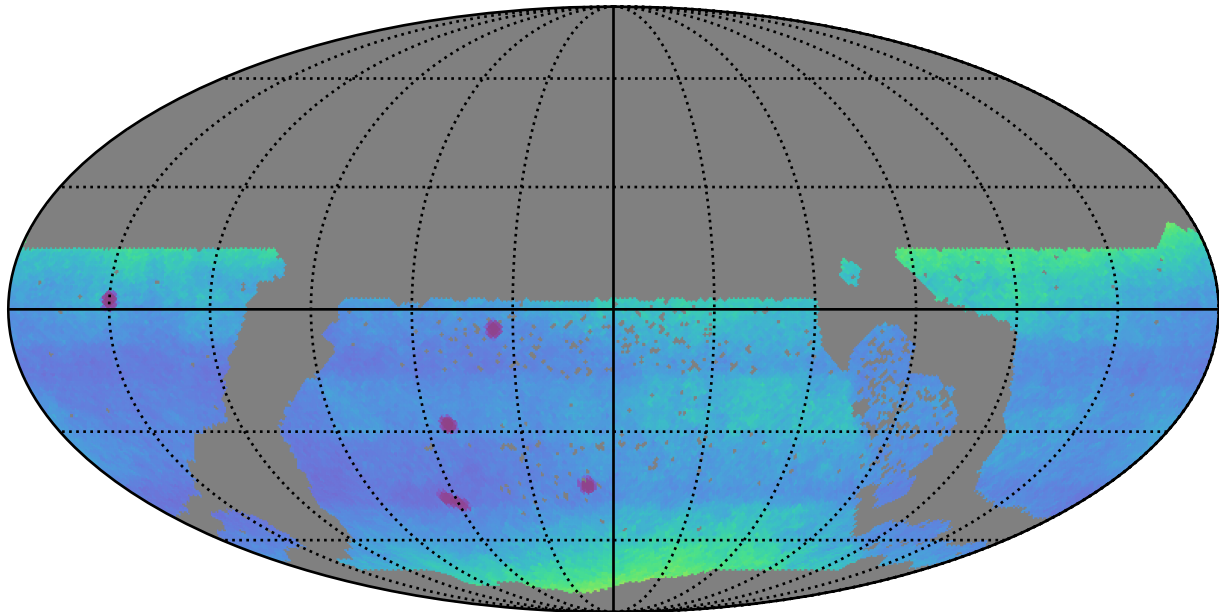
extra_ss_neo7_v3.4_10yrs WFD: Proper Motion Uncert @ 24.0
