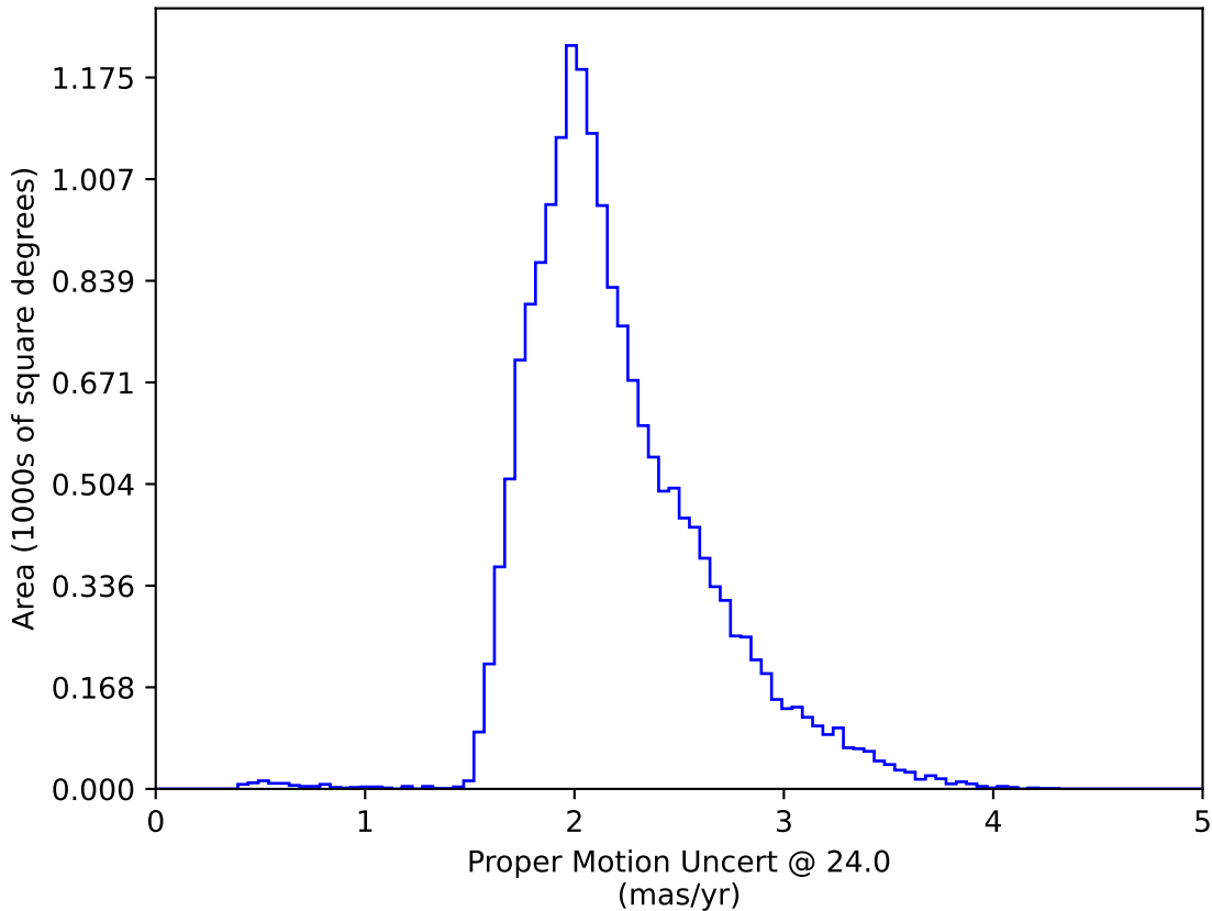
extra_ss_neo7_v3.4_10yrs WFD: Proper Motion Uncert @ 24.0
