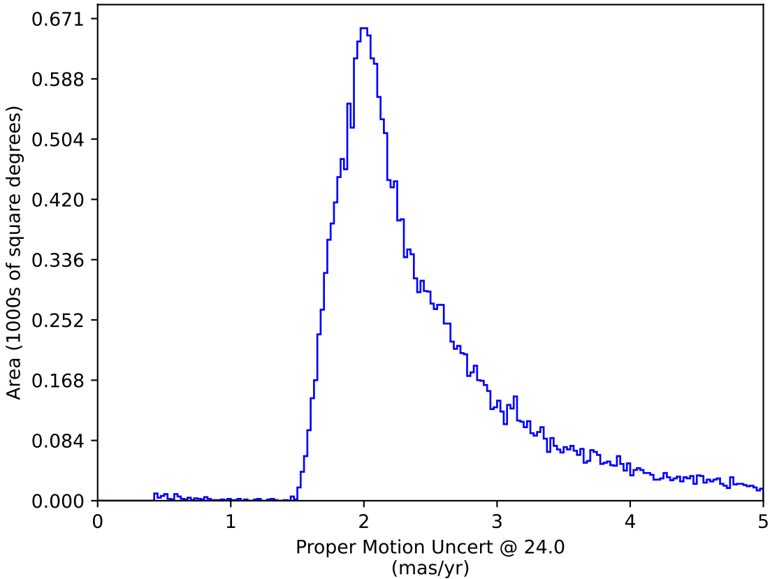
extra_ss_neo7_v3.4_10yrs All sky: Proper Motion Uncert @ 24.0
