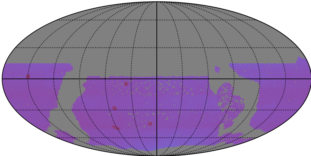
extra_ss_neo7_v3.4_10yrs WFD: Proper Motion Uncert @ 20.5
