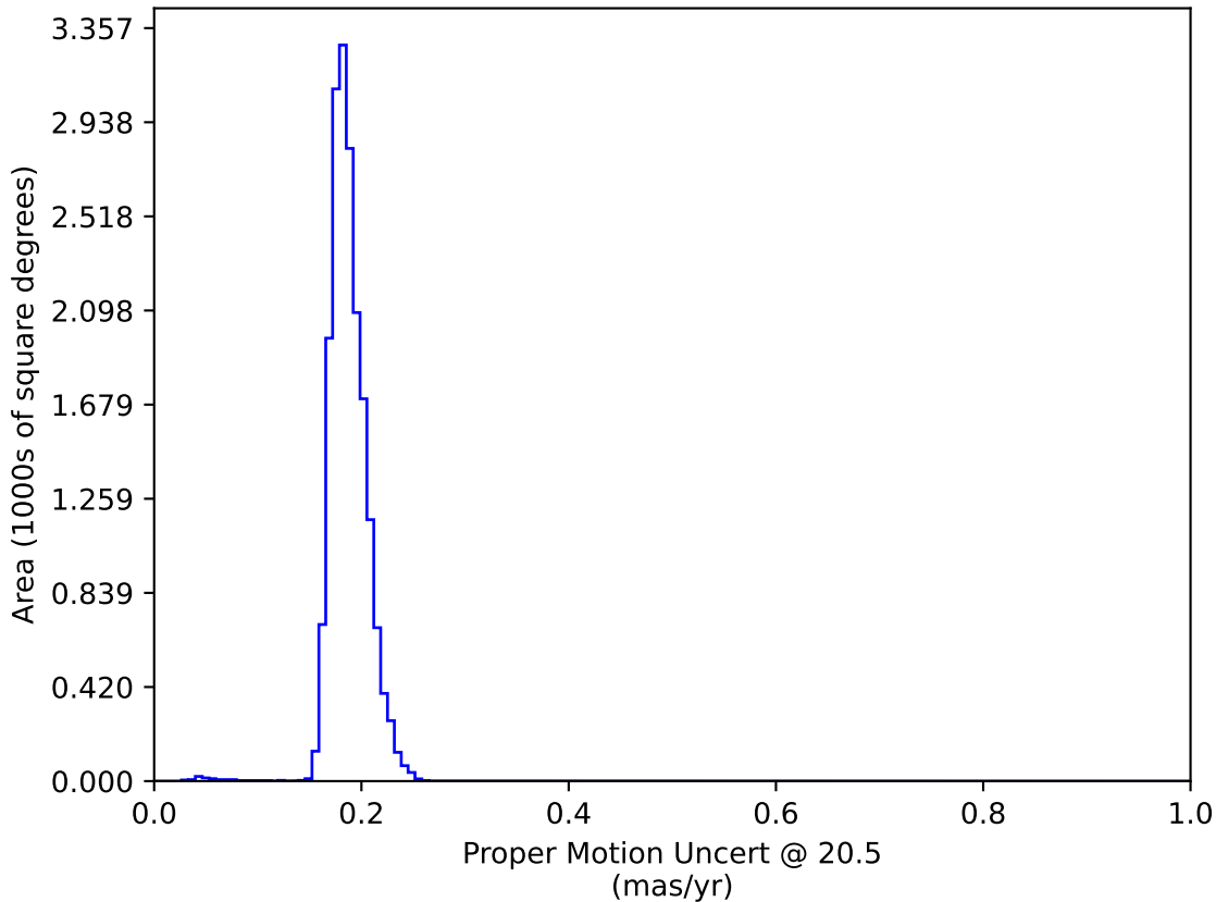
extra_ss_neo7_v3.4_10yrs WFD: Proper Motion Uncert @ 20.5
