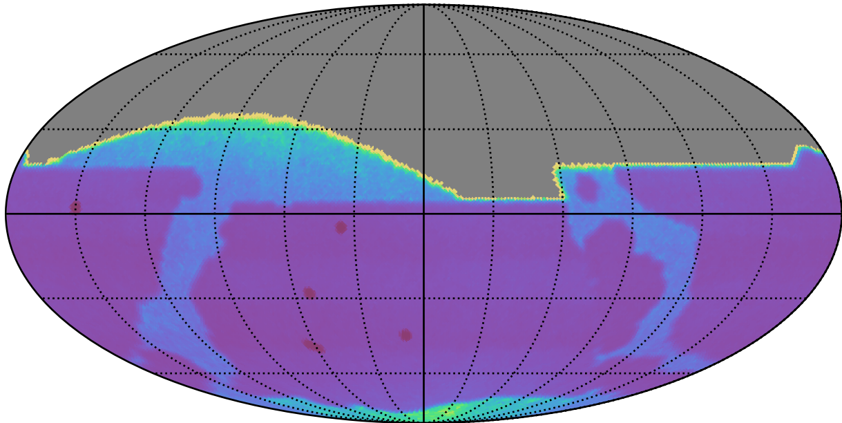
extra_ss_neo7_v3.4_10yrs All sky: Proper Motion Uncert @ 20.5
