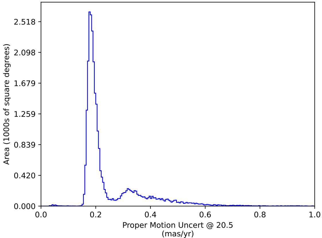
extra_ss_neo7_v3.4_10yrs All sky: Proper Motion Uncert @ 20.5
