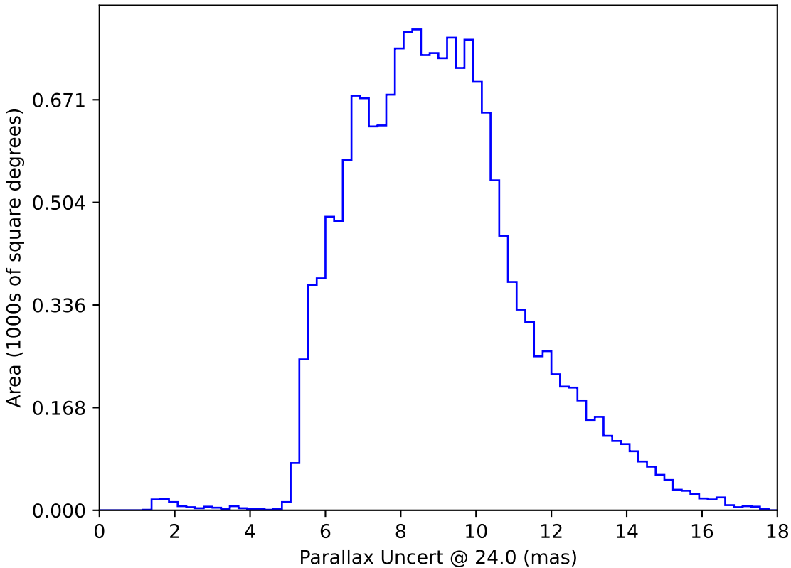
extra_ss_neo7_v3.4_10yrs WFD: Parallax Uncert @ 24.0
