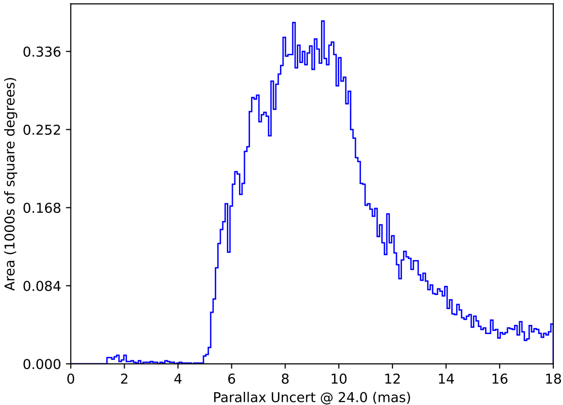
extra_ss_neo7_v3.4_10yrs All sky: Parallax Uncert @ 24.0
