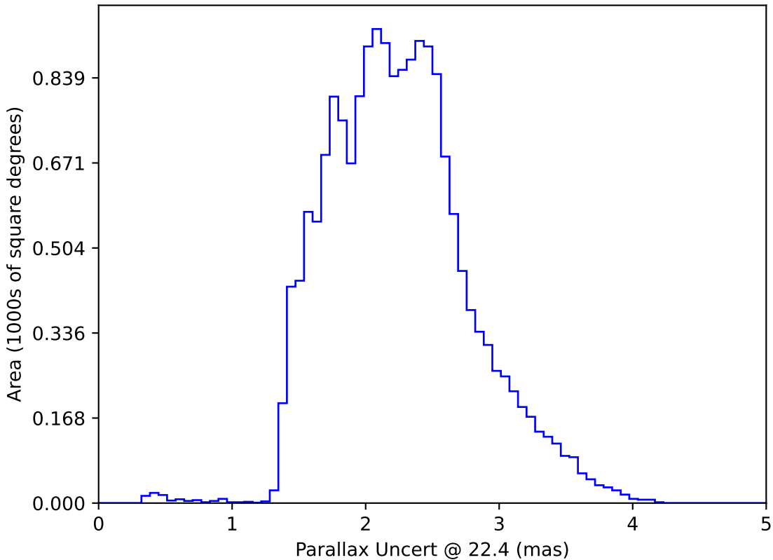
extra_ss_neo7_v3.4_10yrs WFD: Parallax Uncert @ 22.4
