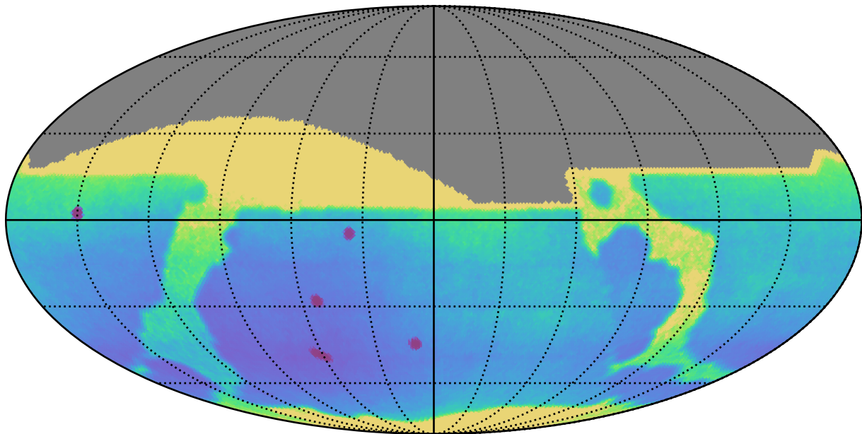
extra_ss_neo7_v3.4_10yrs All sky: Parallax Uncert @ 22.4
