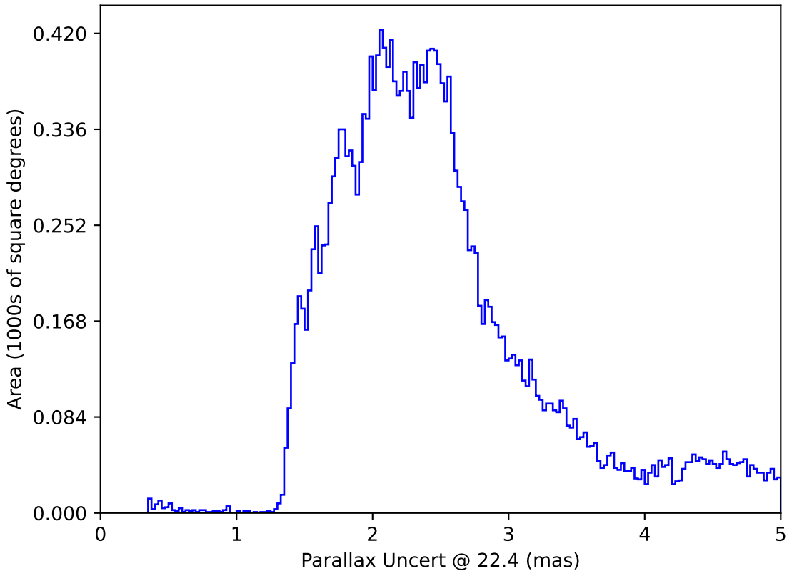
extra_ss_neo7_v3.4_10yrs All sky: Parallax Uncert @ 22.4
