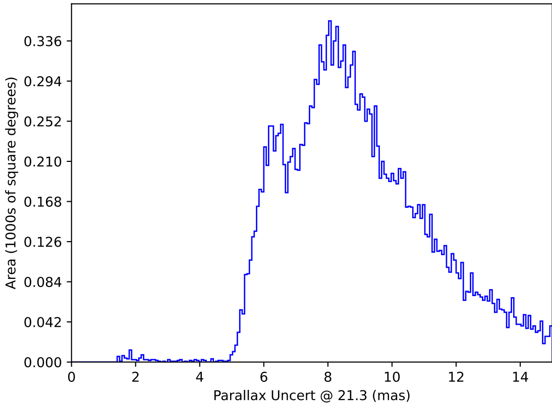
extra_ss_neo7_v3.4_10yrs All sky y band only: Parallax Uncert @ 21.3
