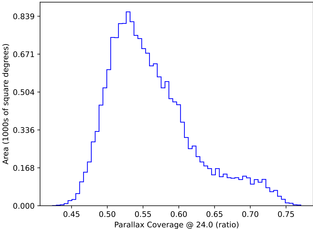
extra_ss_neo7_v3.4_10yrs WFD: Parallax Coverage @ 24.0
