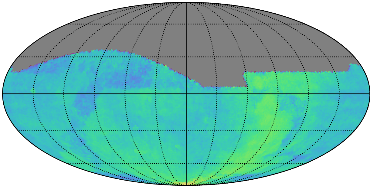
extra_ss_neo7_v3.4_10yrs All sky: Parallax Coverage @ 24.0
