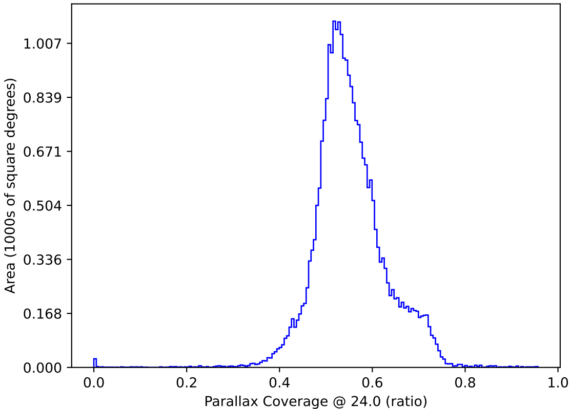
extra_ss_neo7_v3.4_10yrs All sky: Parallax Coverage @ 24.0
