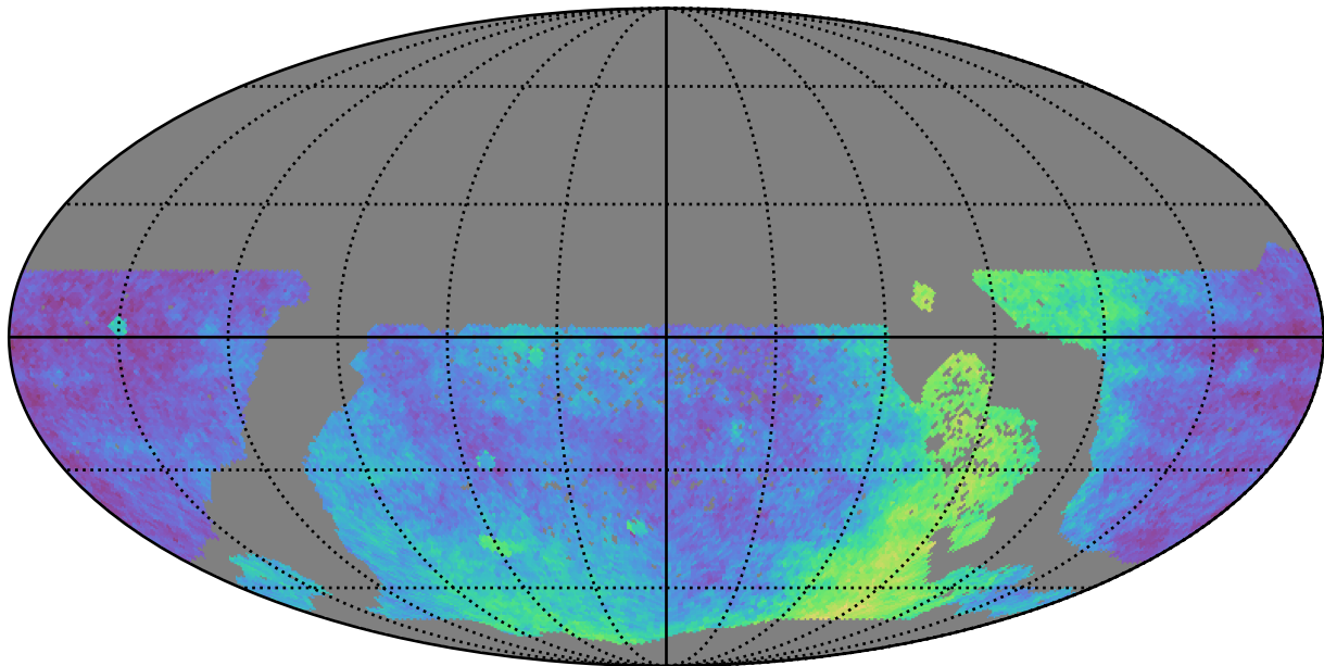
extra_ss_neo7_v3.4_10yrs WFD: Parallax Coverage @ 22.4
