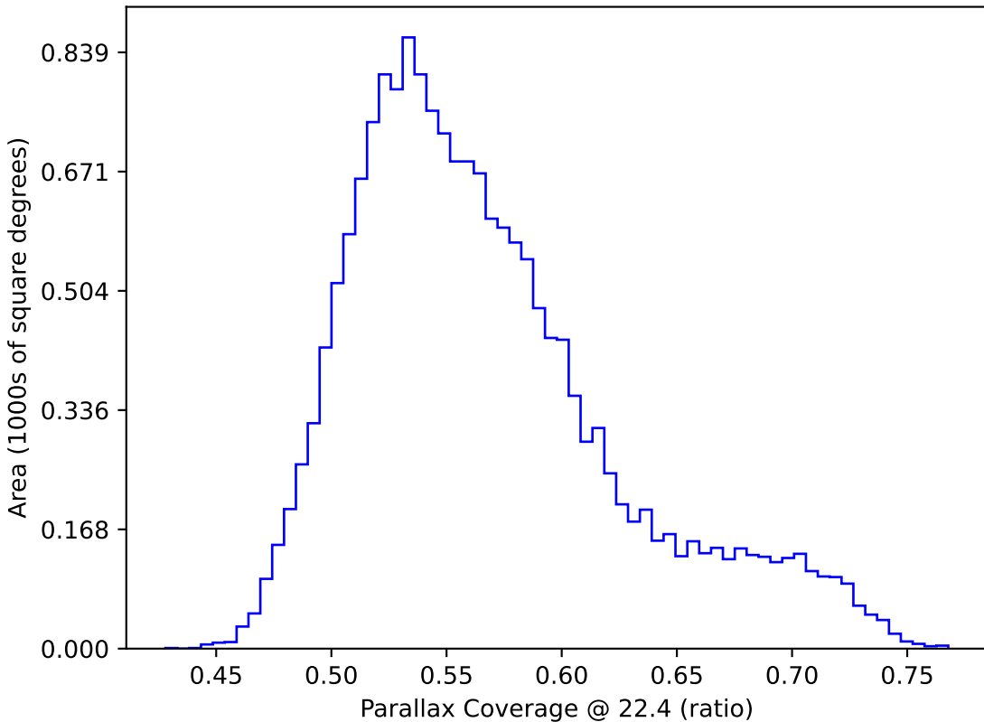
extra_ss_neo7_v3.4_10yrs WFD: Parallax Coverage @ 22.4
