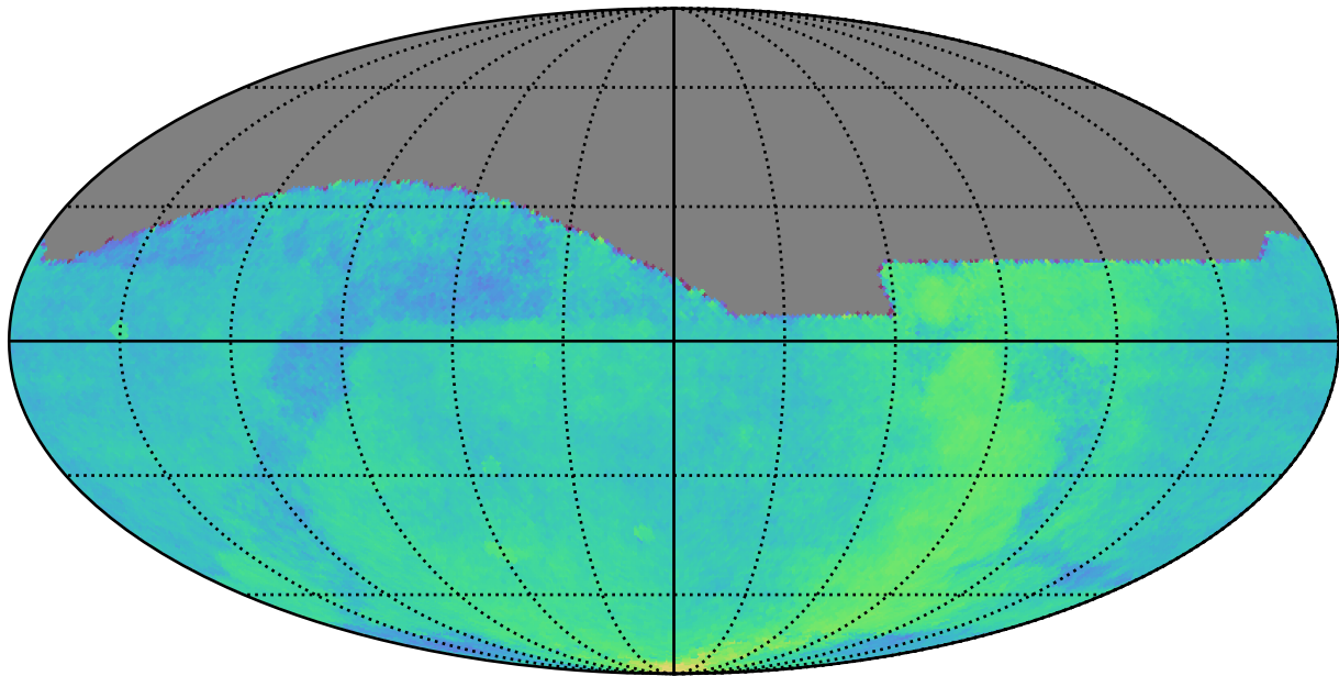
extra_ss_neo7_v3.4_10yrs All sky: Parallax Coverage @ 22.4
