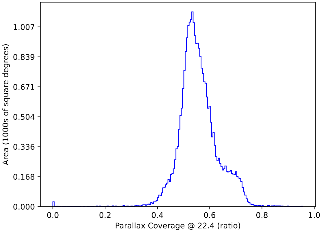
extra_ss_neo7_v3.4_10yrs All sky: Parallax Coverage @ 22.4
