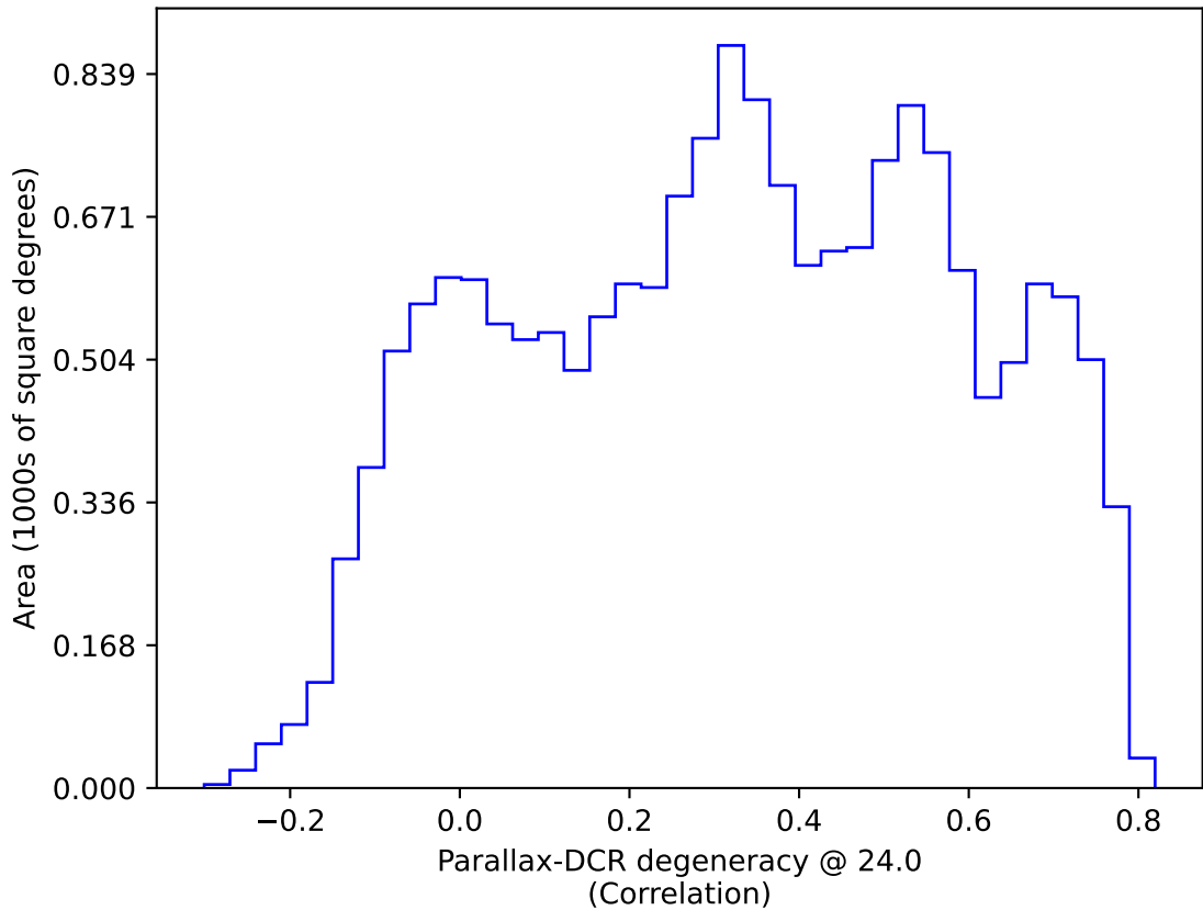
extra_ss_neo7_v3.4_10yrs WFD: Parallax-DCR degeneracy @ 24.0
