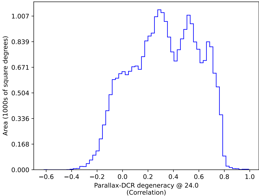
extra_ss_neo7_v3.4_10yrs All sky: Parallax-DCR degeneracy @ 24.0
