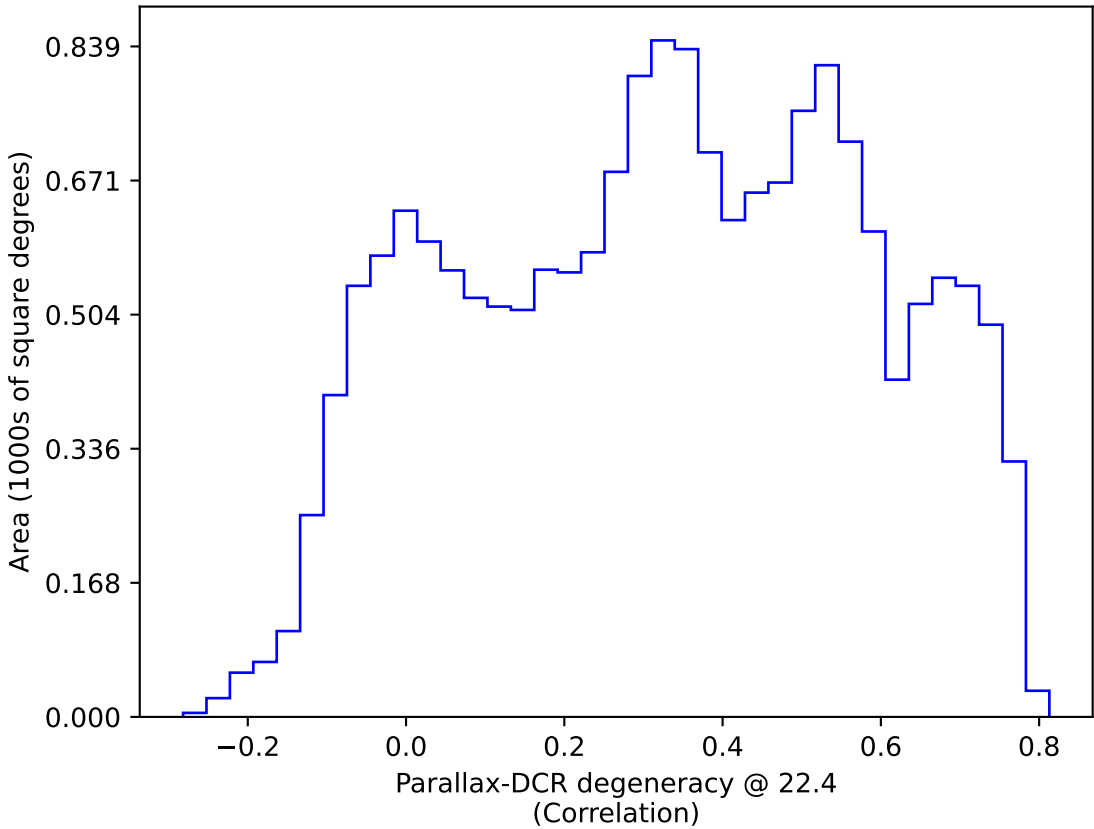
extra_ss_neo7_v3.4_10yrs WFD: Parallax-DCR degeneracy @ 22.4
