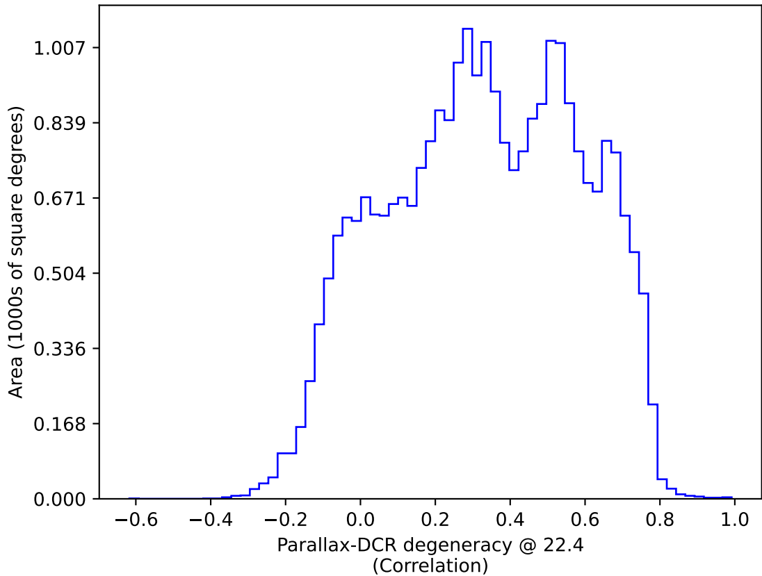
extra_ss_neo7_v3.4_10yrs All sky: Parallax-DCR degeneracy @ 22.4
