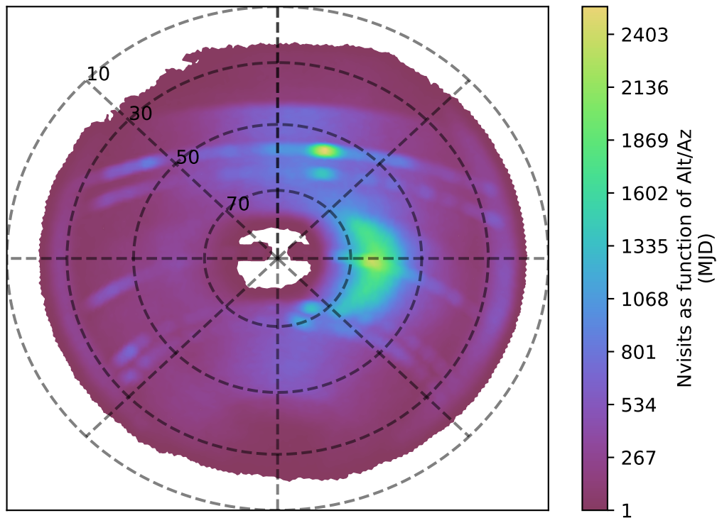
extra_ss_neo7_v3.4_10yrs z band: Nvisits as function of Alt/Az
