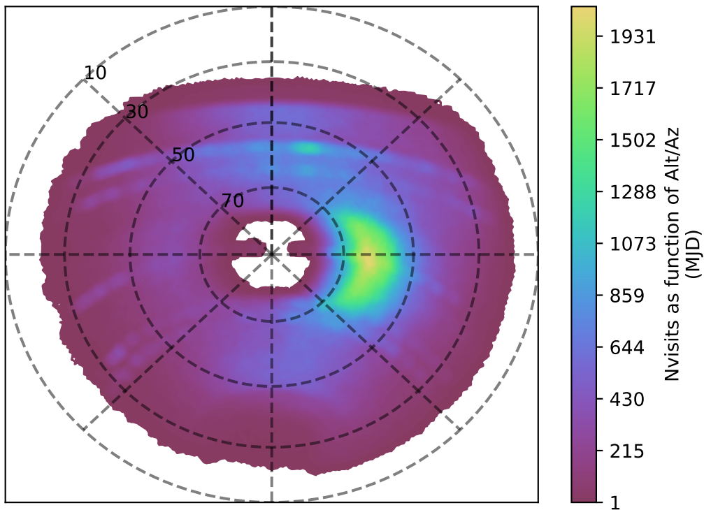
extra_ss_neo7_v3.4_10yrs y band: Nvisits as function of Alt/Az
