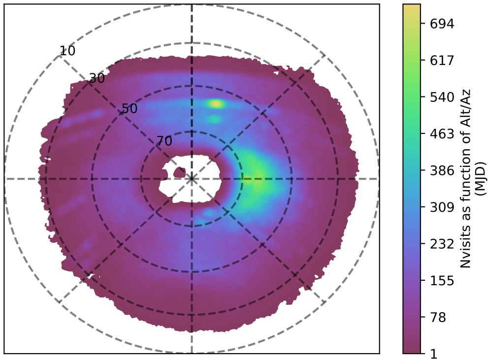
extra_ss_neo7_v3.4_10yrs u band: Nvisits as function of Alt/Az
