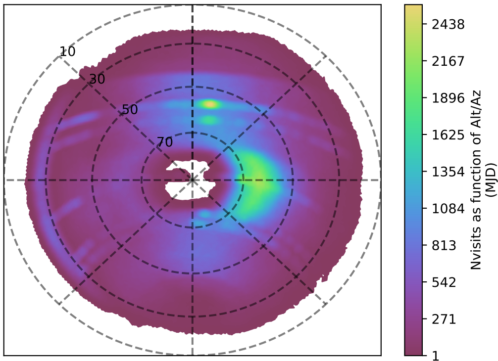
extra_ss_neo7_v3.4_10yrs r band: Nvisits as function of Alt/Az
