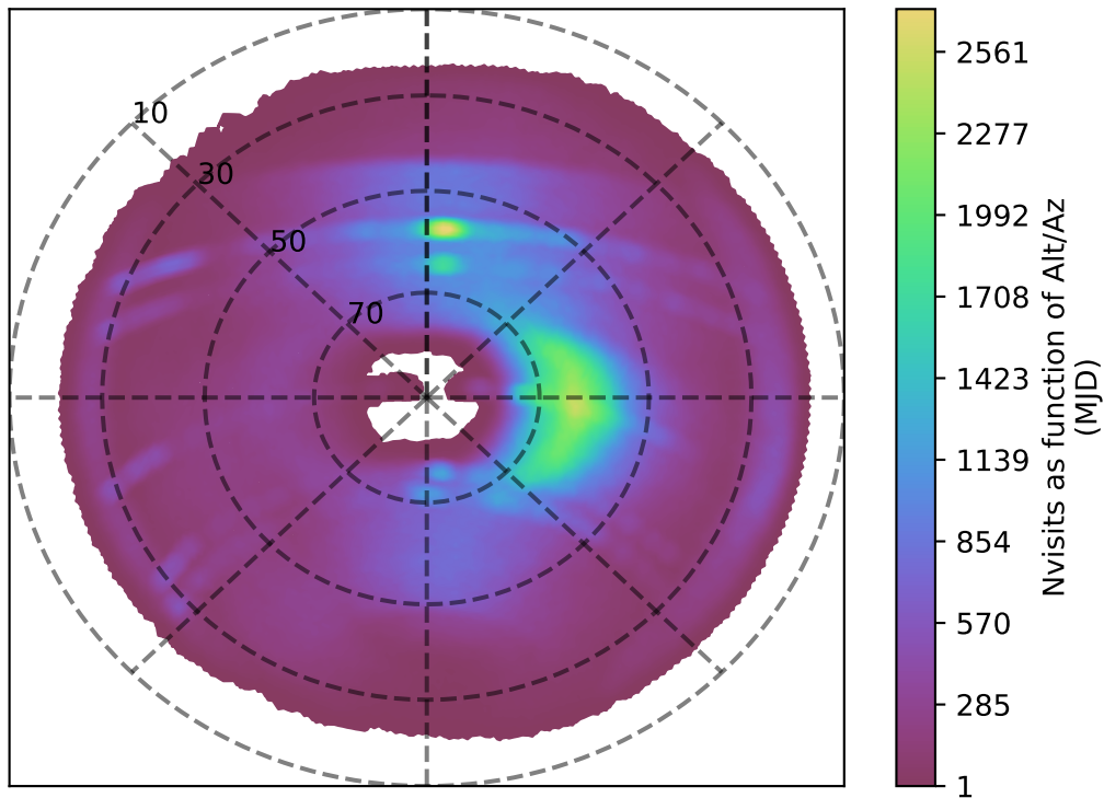
extra_ss_neo7_v3.4_10yrs i band: Nvisits as function of Alt/Az
