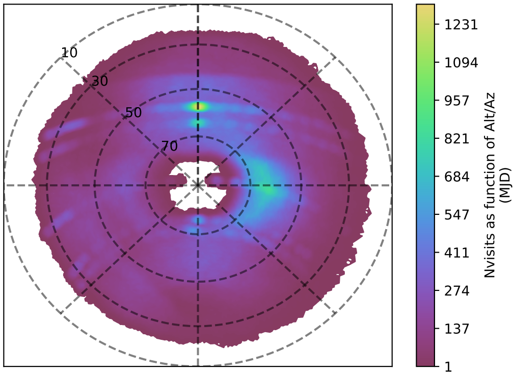
extra_ss_neo7_v3.4_10yrs g band: Nvisits as function of Alt/Az
