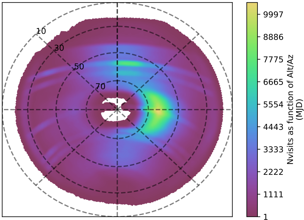
extra_ss_neo7_v3.4_10yrs all bands: Nvisits as function of Alt/Az
