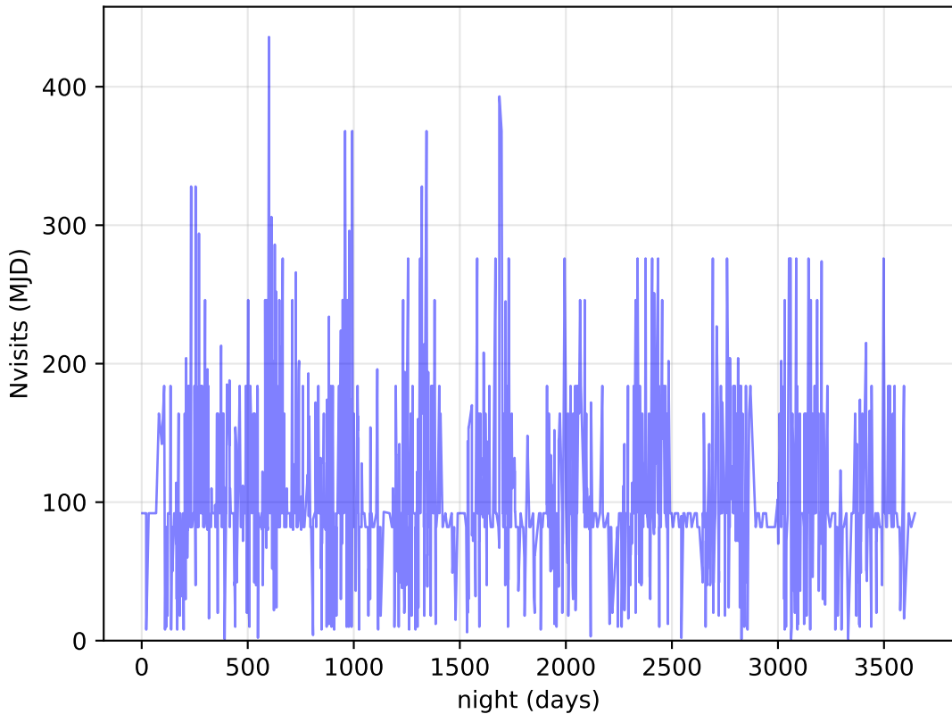
extra_ss_neo7_v3.4_10yrs DDF: Nvisits
