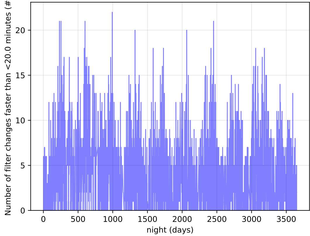
extra_ss_neo7_v3.4_10yrs Per Night: Number of filter changes faster than <20.0 minutes
