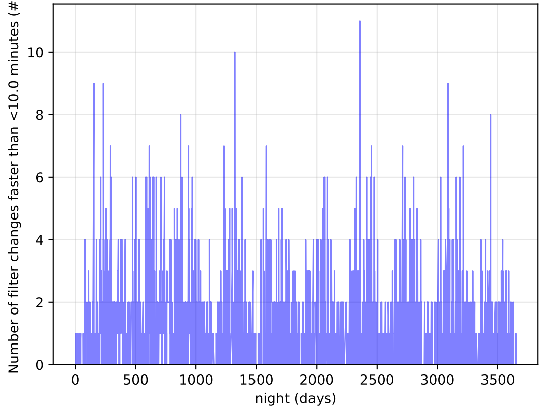
extra_ss_neo7_v3.4_10yrs Per Night: Number of filter changes faster than <10.0 minutes
