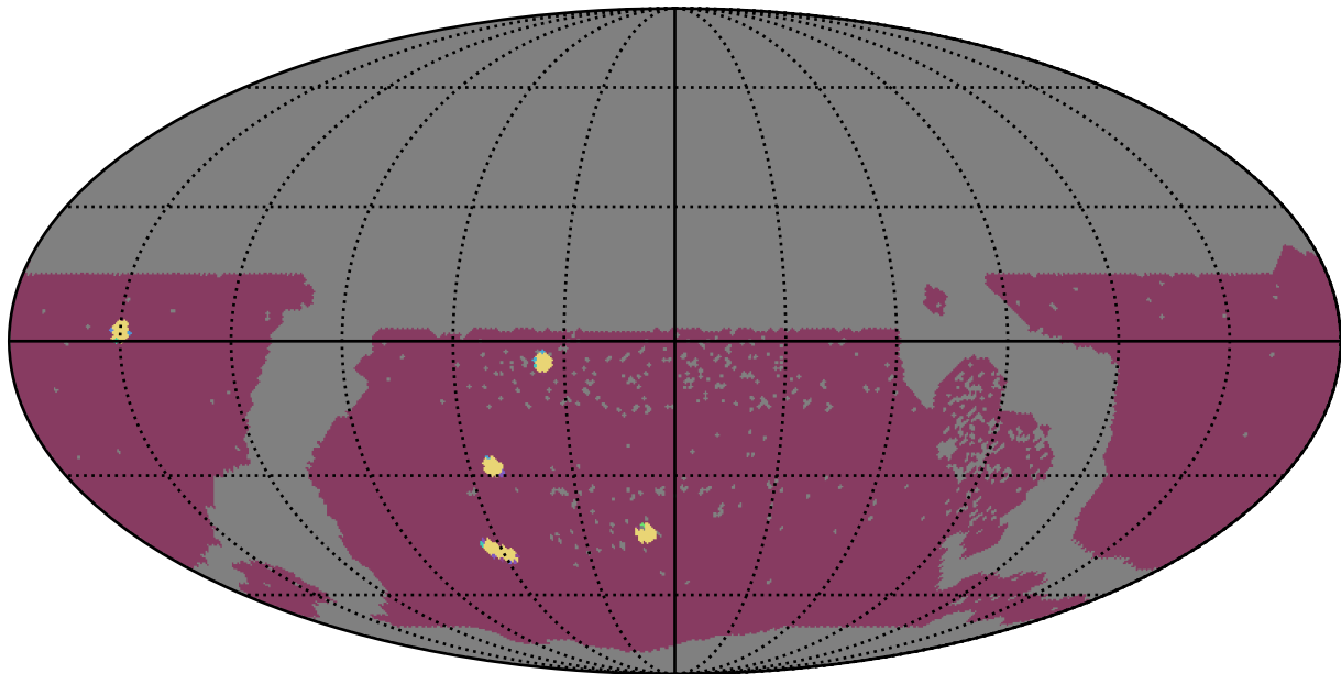
extra_ss_neo7_v3.4_10yrs WFD: NumberOfQuickRevisits
