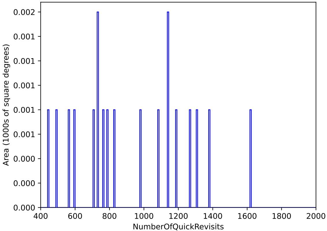
extra_ss_neo7_v3.4_10yrs WFD: NumberOfQuickRevisits
