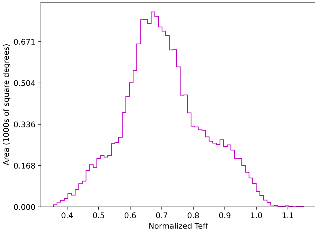
extra_ss_neo7_v3.4_10yrs WFD z band: Normalized Teff
