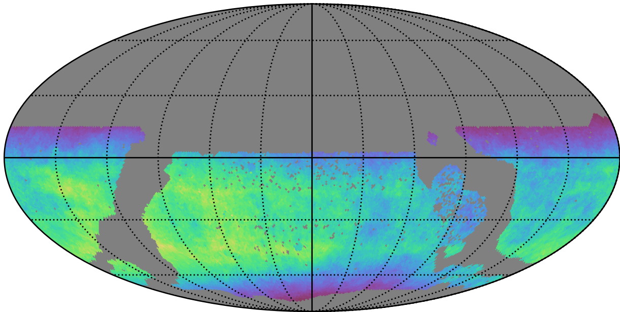
extra_ss_neo7_v3.4_10yrs WFD y band: Normalized Teff
